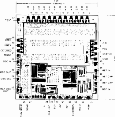
Chip Topography
