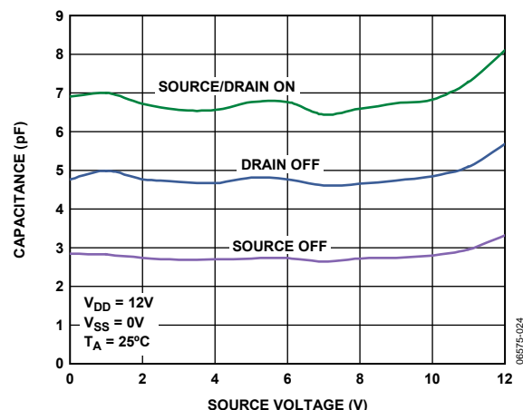
Figure 20. Capacitance vs. Source Voltage for Single Supply
