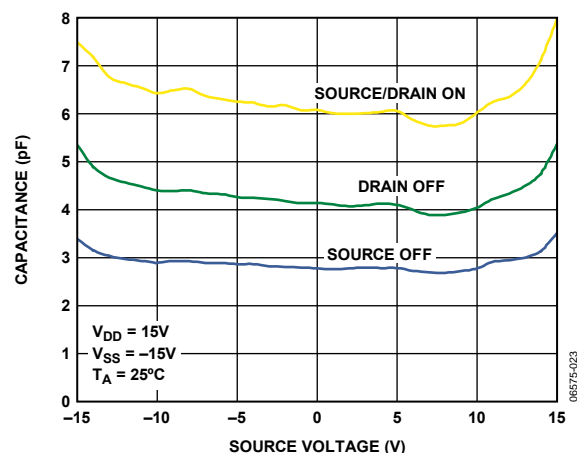
Figure 19. Capacitance vs. Source Voltage for Dual Supply
