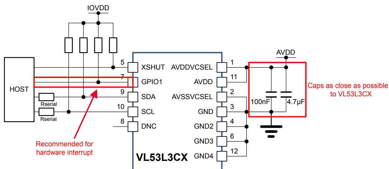
Figure 3. VL53L3CX schematic
