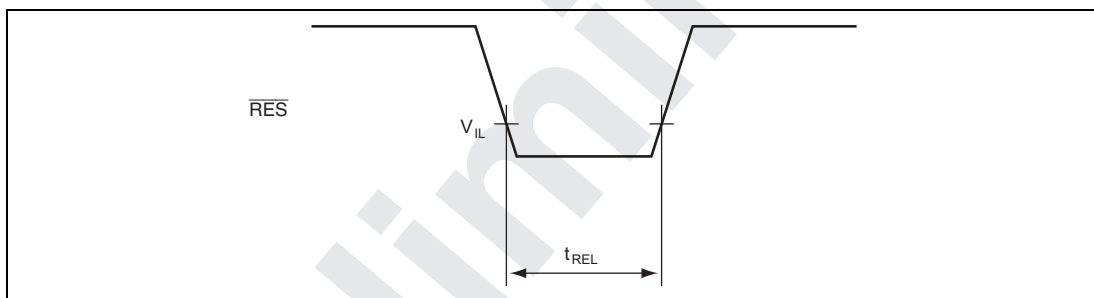
Figure 24.3 \overline{RES} Low Width Timing
