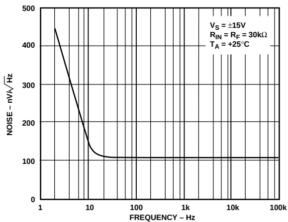
Figure 10. Voltage Noise Density vs. Frequency, Class AB
