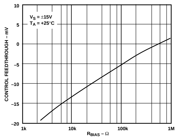
Figure 13. Control Feedthrough vs. R_{BIAS}
