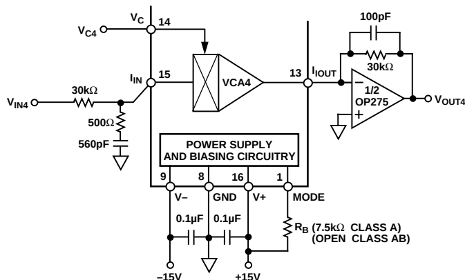
Figure 1. R_{IN} = R_{OUT} = 30 k \Omega , C_F = 100 pF. Optional R_B = 7.5 k \Omega , Biases Gain Core to Class A Operation. For Class AB, Omit R_B .
