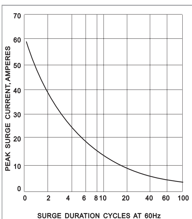
FIG.4-NON-RECURRENT SURGE RATING
