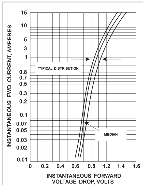
FIG.2-TYPICAL FORWARD CHARACTERISTICS (25°C)
