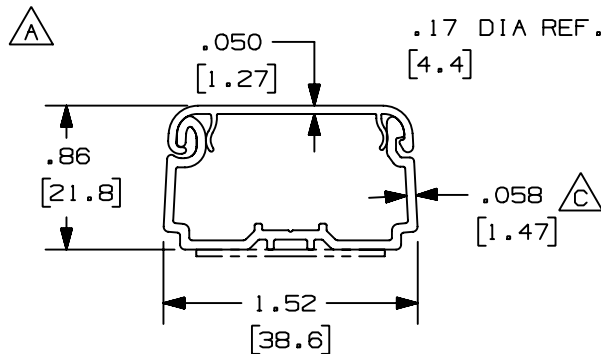
LDPH10 CLOSED POSITION
