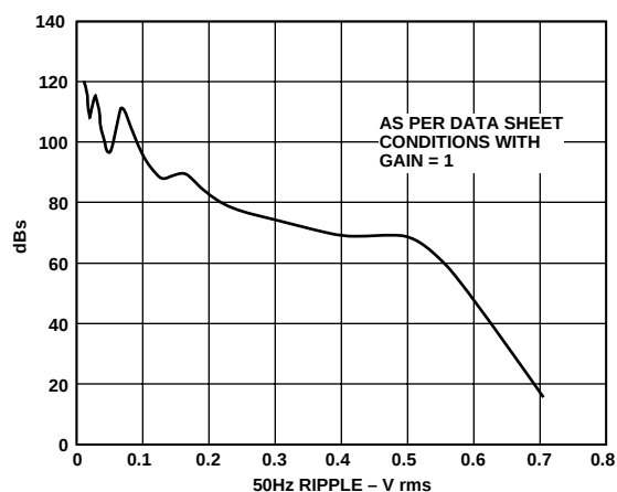
Figure 1. PSR as a Function of V DD 50 Hz Ripple
