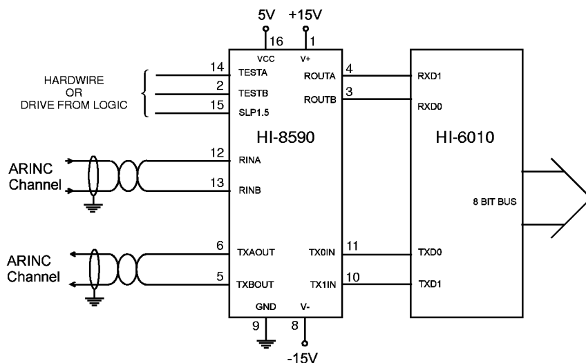
FIGURE 3 - APPLICATION DIAGRAM
