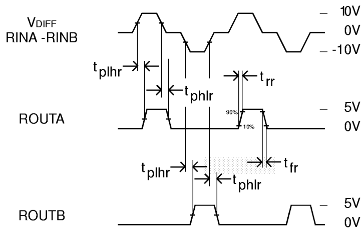
FIGURE 5 - RECEIVER TIMING
