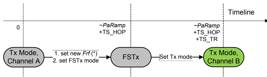
Figure 13. Transmitter Hopping
