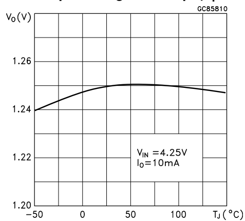
Figure 5. Output voltage vs. temp. ( V_I = 4.25\ \text{V} )
