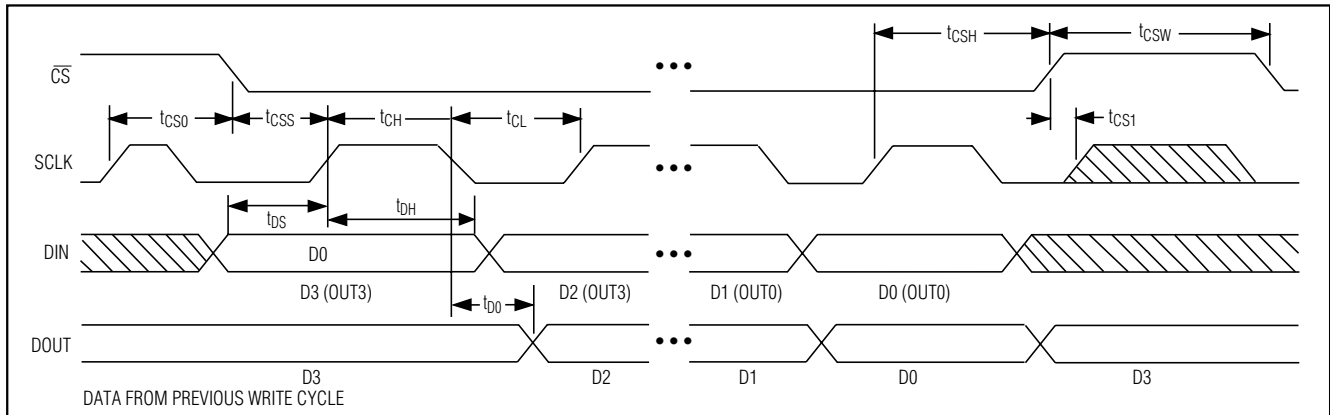
Figure 6. Serial-Mode Timing
