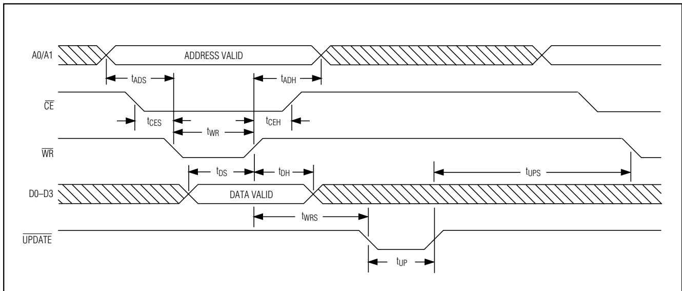
Figure 4. Parallel-Mode Timing
