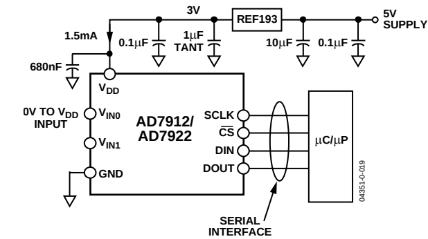
Figure 22. REF193 as Power Supply to AD7912/AD7922
