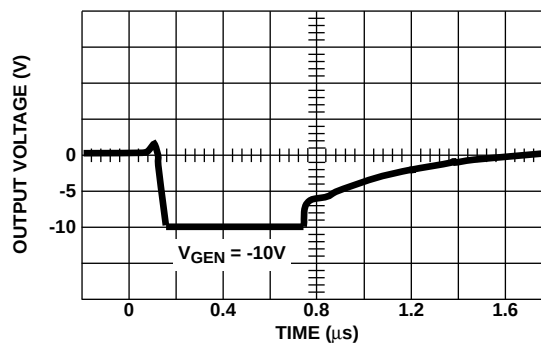
7H. V_{OUT} vs TIME
