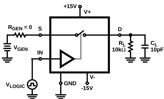
7A. TEST CIRCUIT
