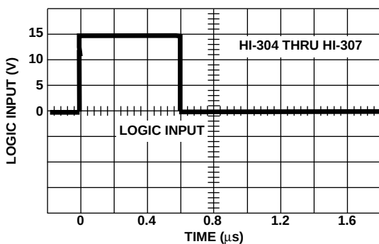
7C. V_{IN(Logic)} vs TIME
