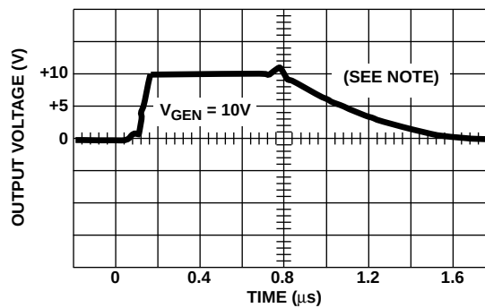
7D. V_{OUT} vs TIME
