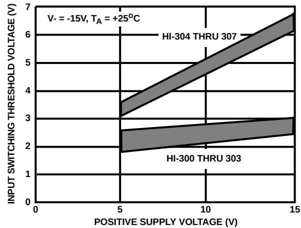
FIGURE 16. INPUT SWITCHING THRESHOLD vs POSITIVE SUPPLY VOLTAGE, HI-300 THRU HI-307
