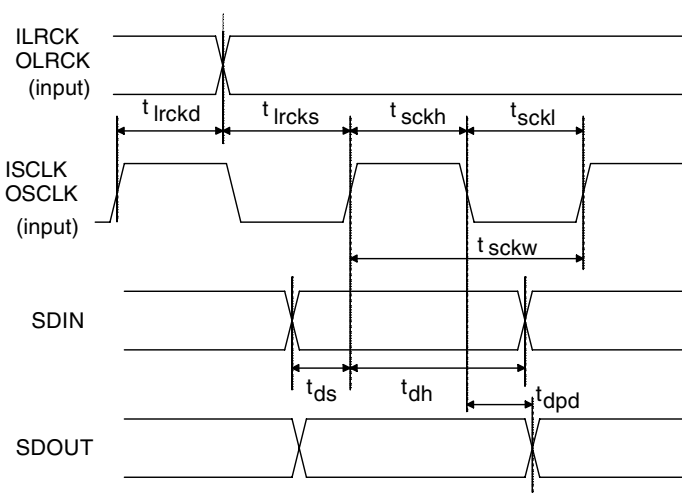
Figure 2. Audio Port Slave Mode and Data Input Timing
