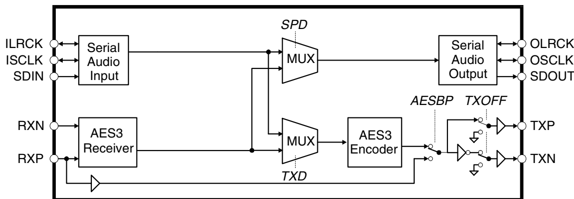
Figure 9. Software Mode Audio Data Flow Switching Options
