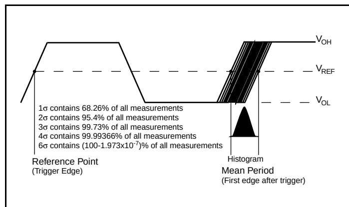
Period Jitter
