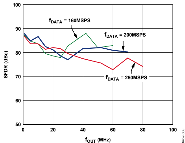
Figure 9. AD9779A In-Band SFDR vs. f_{OUT} , 2x Interpolation
