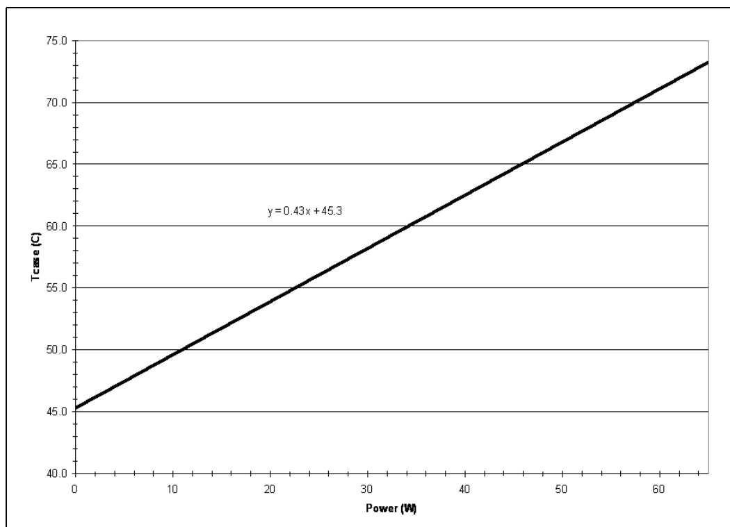
Figure 16. Thermal Profile (Intel® Pentium® Dual-Core Processors with CPUID = 06FDh)
