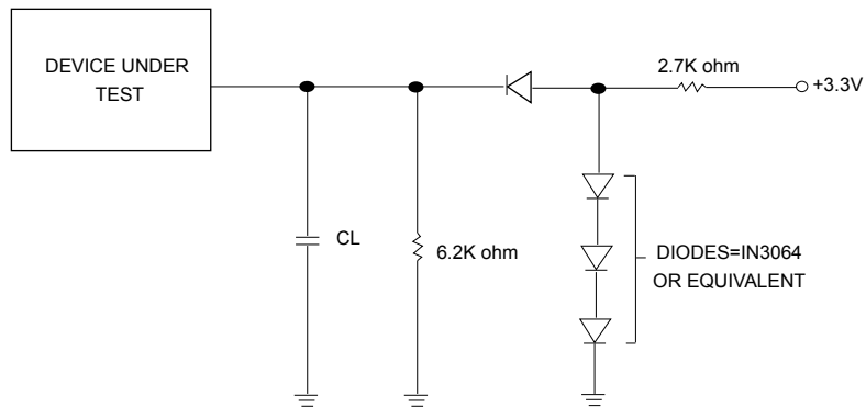
Figure 46. OUTPUT LOADING
