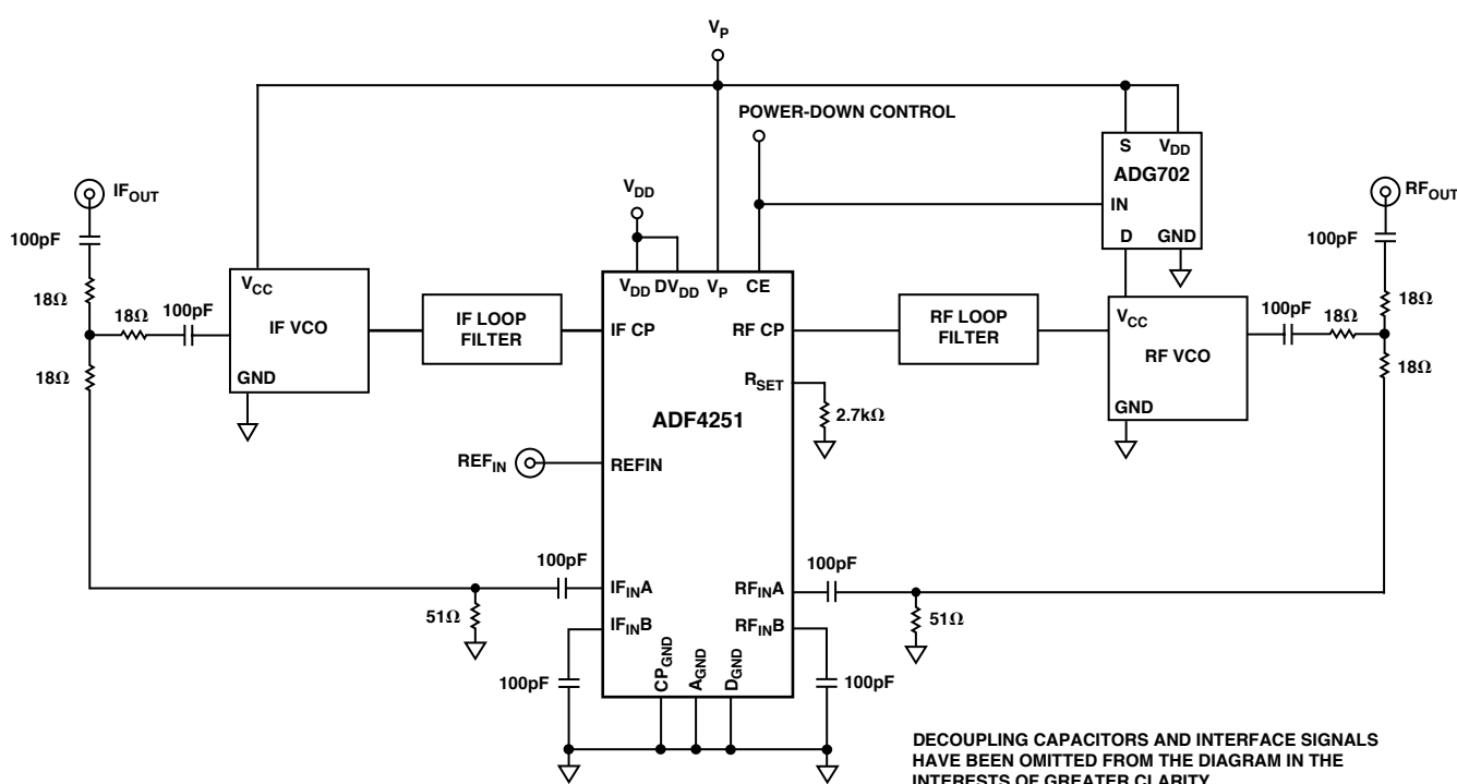
Figure 9. Power-Down Circuit
