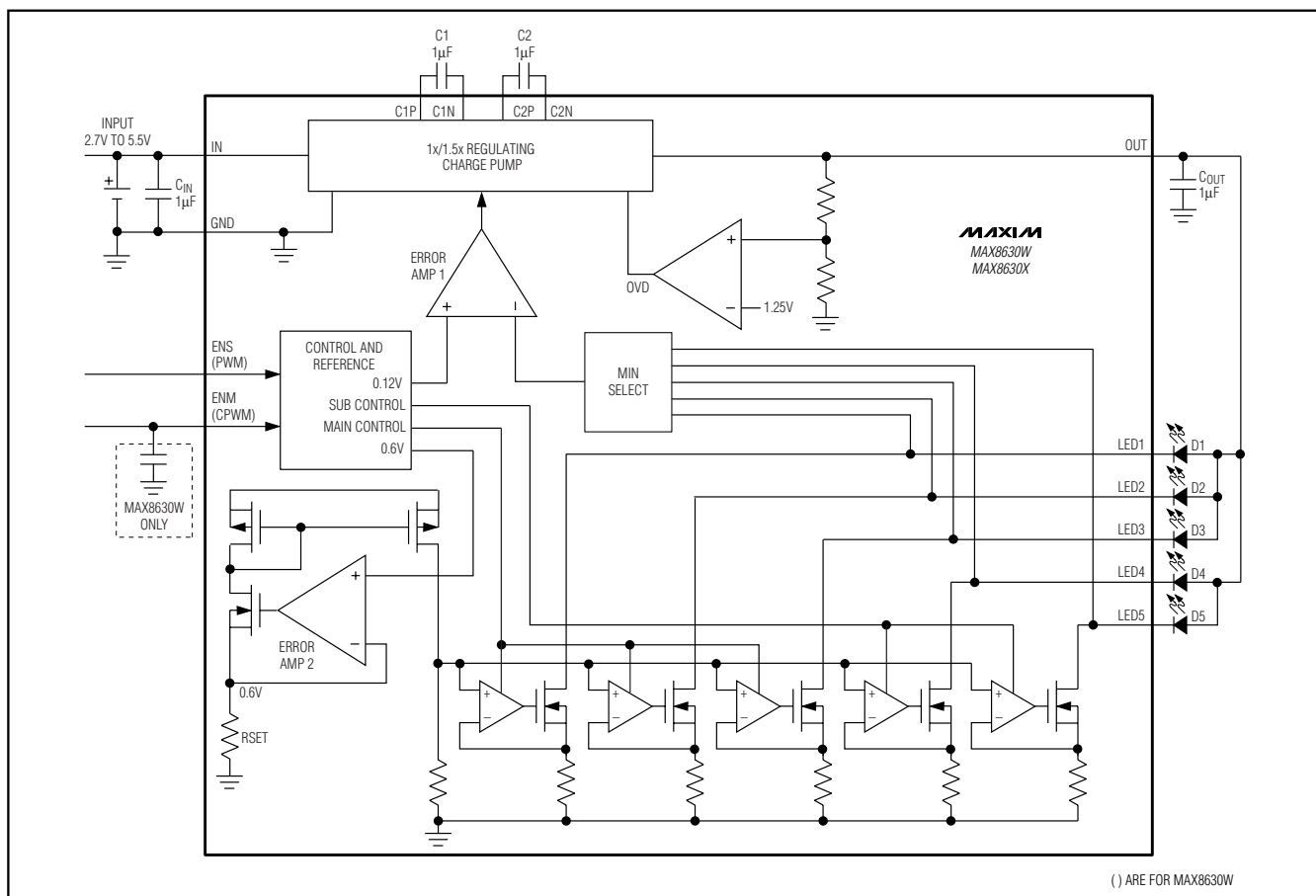
Figure 3. Functional Diagram
