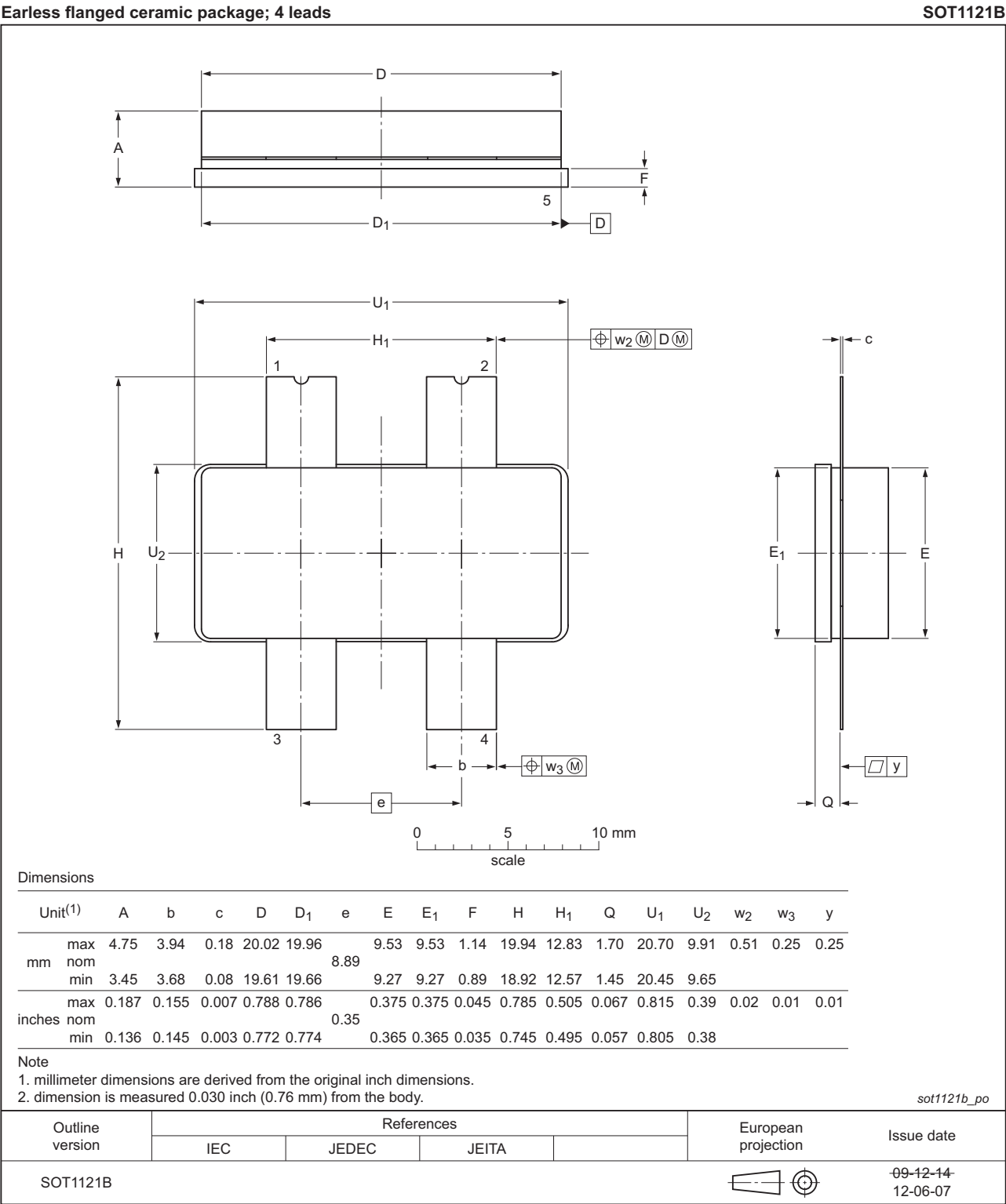
Fig 7. Package outline SOT1121B
