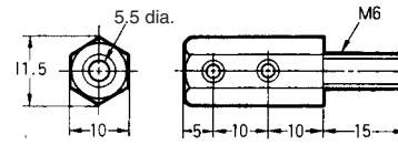
F03-06 Electrode Band Connecting Nut (SUS304)
