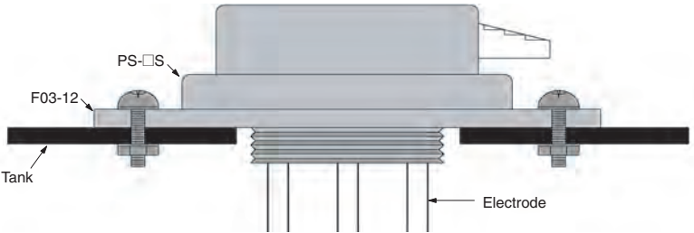
Screw (attached to F03-12)
