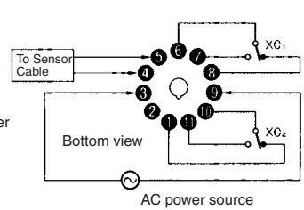
61F-GPN-V50 Water Leak Detector
