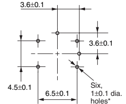
PCB Mounting (Top View)
