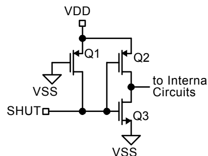
Figure 6. SHUT Pin
