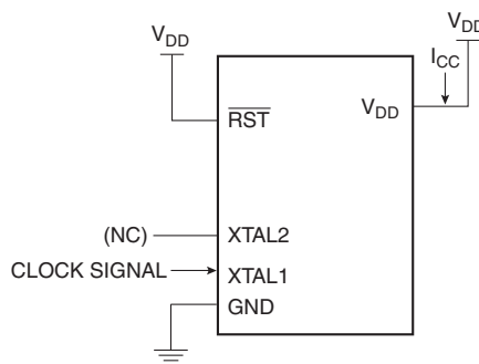
Figure 26-27. Connection Diagram for I_{CC} Idle Measurement. All Other Pins are Disconnected
