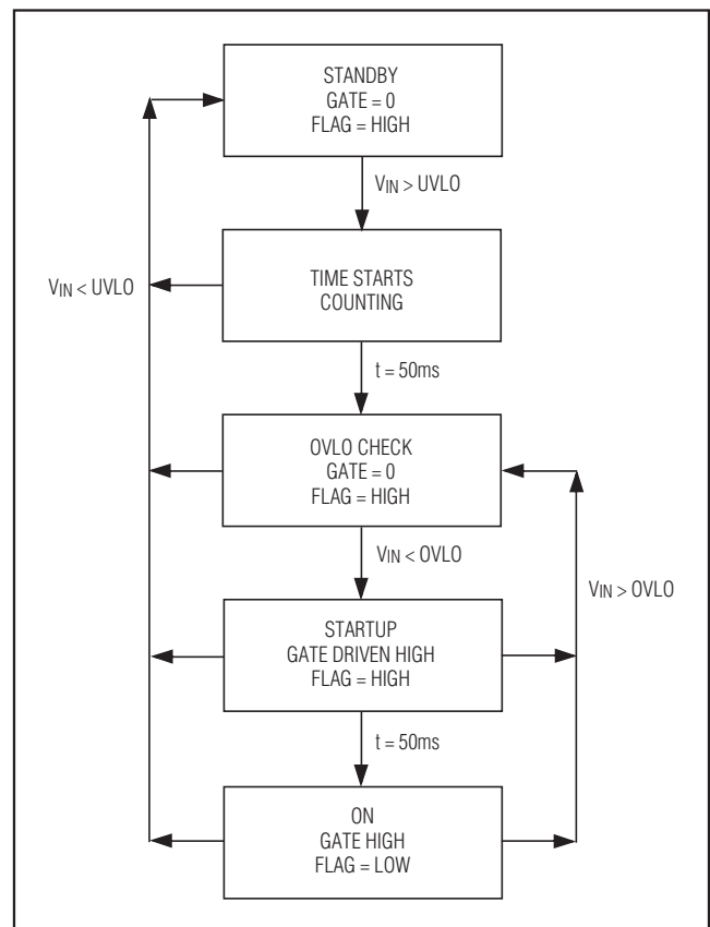
Figure 4. State Diagram
