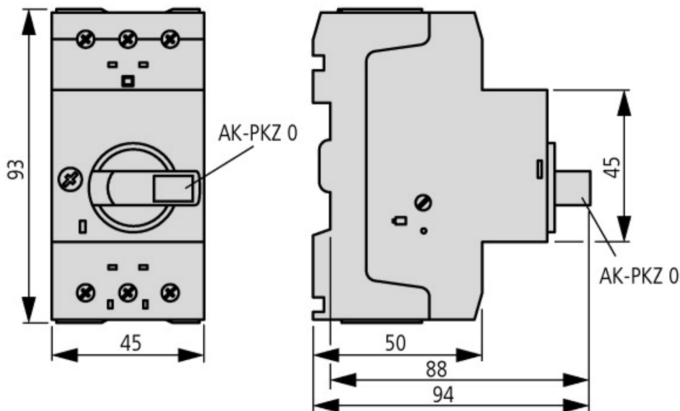
Motor-protective circuit-breakers with lockable rotary handles PKZM0-...+AK-PKZ0
