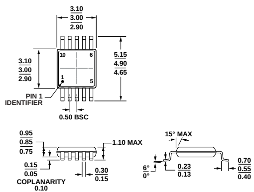
Figure 64. 10-Lead Mini Small Outline Package [MSOP] (RM-10)
