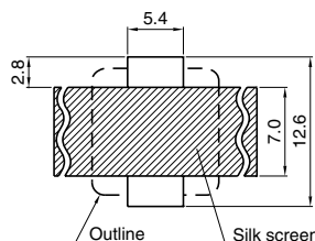
LAND PATTERNS(mm)
