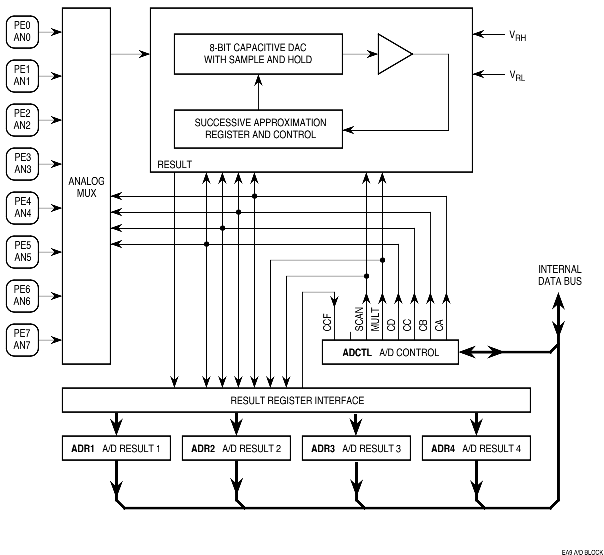
Figure 14 A/D Converter Block Diagram
