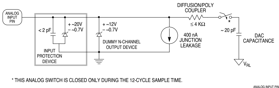
Figure 16 Electrical Model of an Analog Input Pin (Sample Mode)
