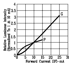
Fig4. RELATIVE LUMINOUS INTENSITY VS. FORWARD CURRENT
