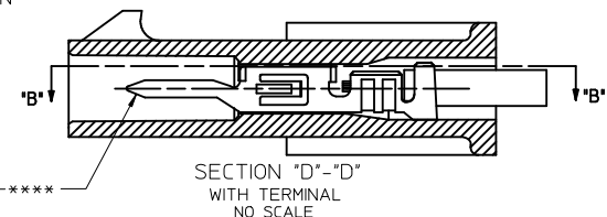
TERMINAL STOPS
