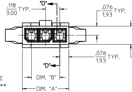
PLUG # 43640-****
