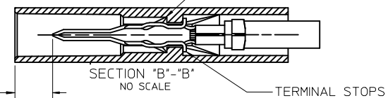
TERMINAL STOPS
