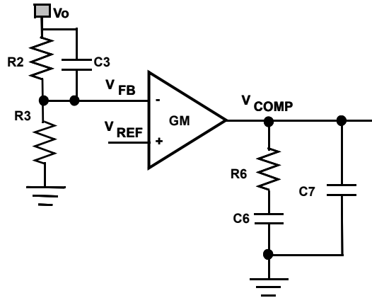
FIGURE 42. TYPE II COMPENSATOR
