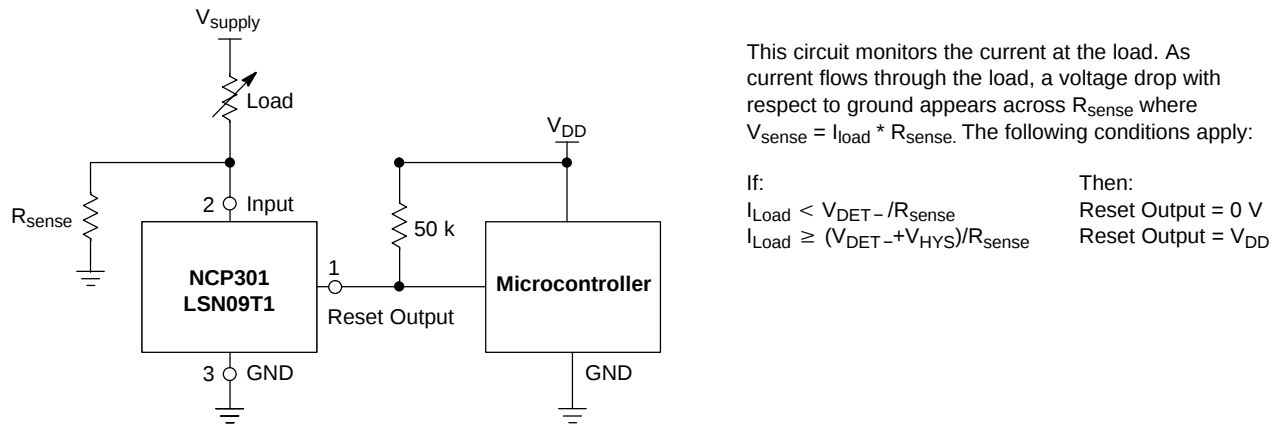
Figure 31. Microcontroller System Load Sensing
