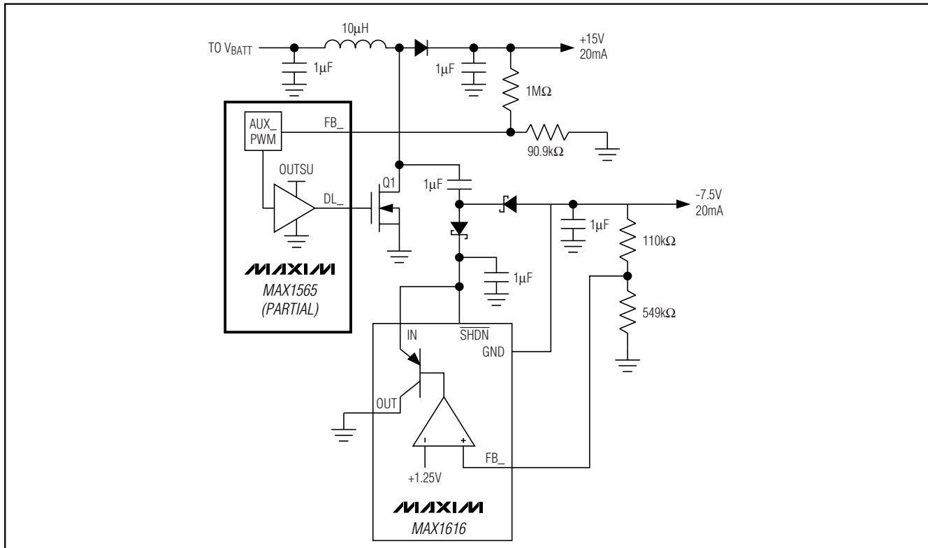
Figure 10. +15\text{V} and -7.5\text{V} CCD Bias without Transformer
