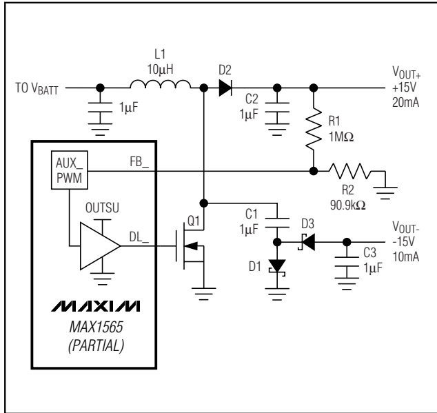
Figure 9. \pm 15\text{V} Output Using a Boost with Charge-Pump Inversion
