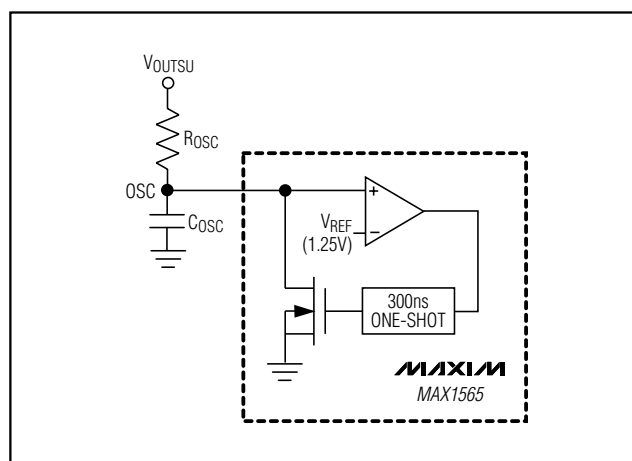
Figure 4. Master Oscillator
