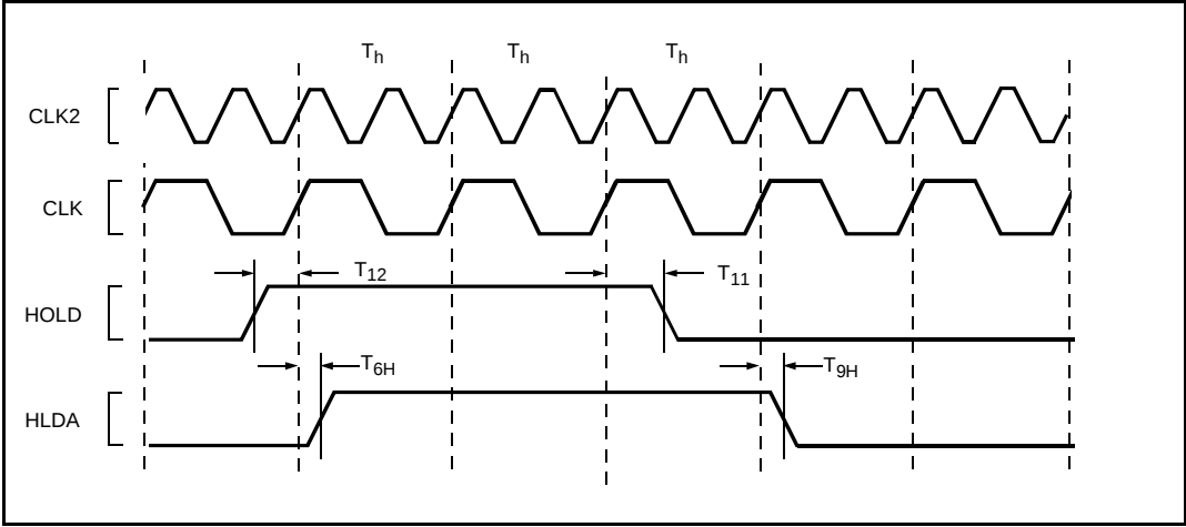
Figure 22. HOLD Timing
