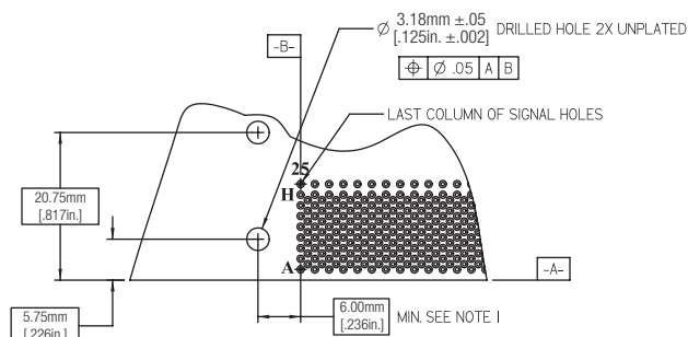
RECOMMENDED PCB HOLE MOUNTING PATTERN (REFERENCED TO A TYPICAL HSHM CONNECTOR FOOTPRINT)
