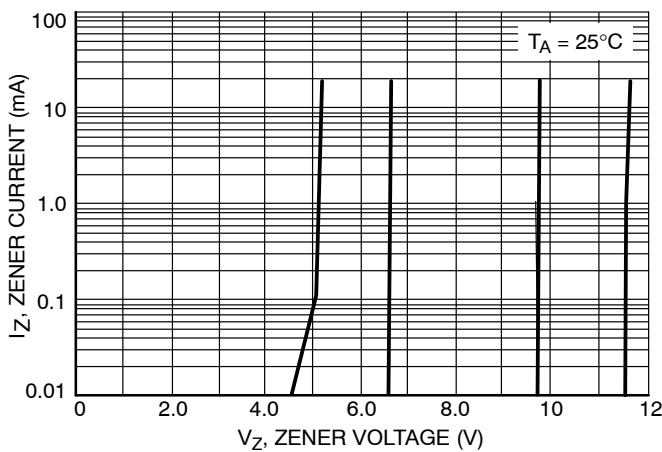
Figure 5. Zener Voltage versus Zener Current ( V_Z Up to 12 \text{ V} )
