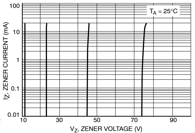
Figure 6. Zener Voltage versus Zener Current ( 12 \text{ V} to 75 \text{ V} )
