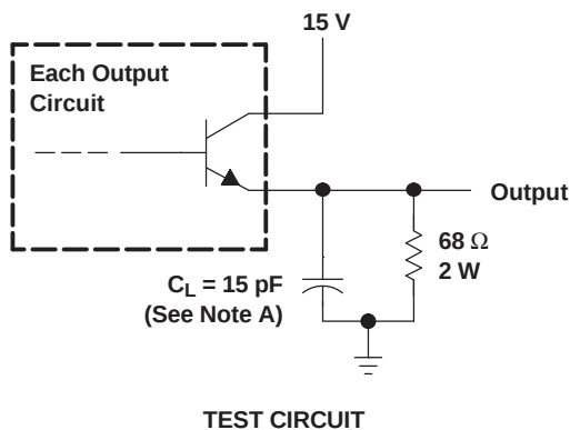
Figure 4. Emitter-Follower Configuration
