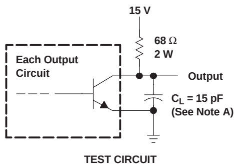
Figure 3. Common-Emitter Configuration
