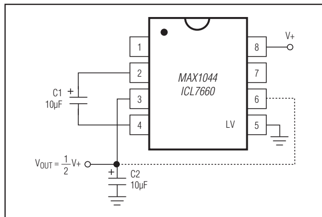
Figure 10. Voltage Divider
