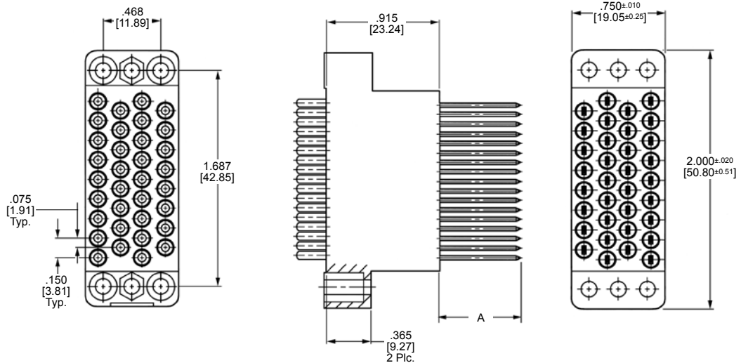
Plug Assembly
