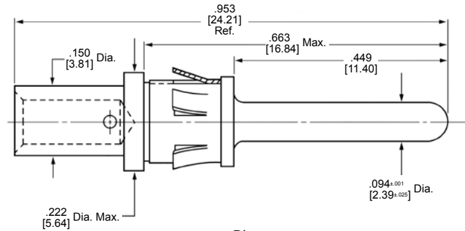
Pin
