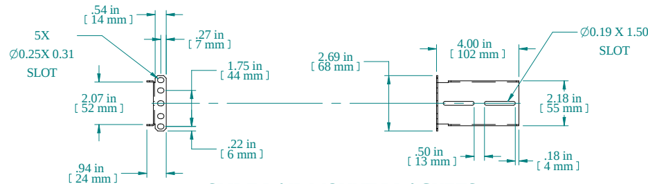
SLIDE RAIL MOUNT BRACKETS
