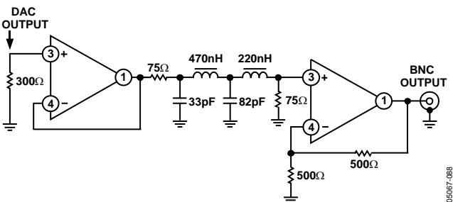
Figure 88. Example of Output Filter for HDTV, 2 \times Oversampling
