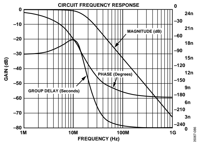
Figure 86. Filter Plot for Output Filter for SD, 16 \times Oversampling
