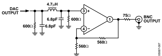
Figure 87. Example of Output Filter for PS, 8 \times Oversampling
