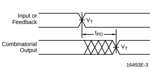
a. Combinatorial output
