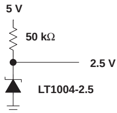
Figure 22. 2.5-V Reference
