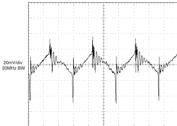
UWR-3.3/9-D24A Output Ripple and Noise (PARD)
