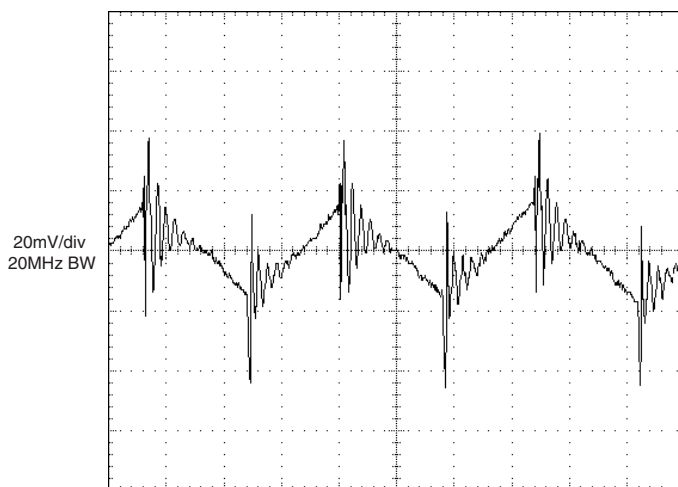
UWR-3.3/9-D48A Output Ripple and Noise (PARD)
