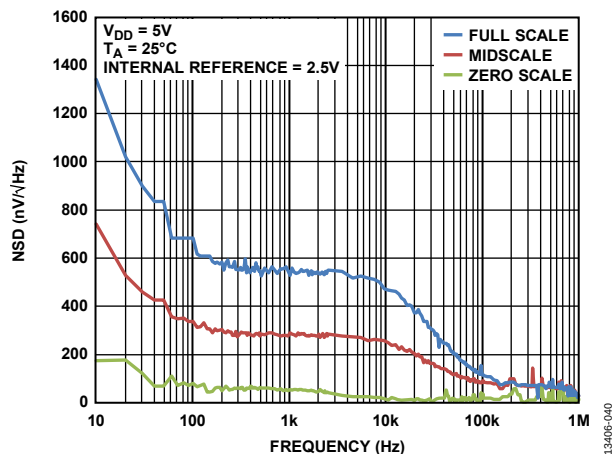
Figure 35. Noise Spectral Density (NSD) vs. Frequency
