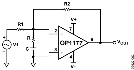
Figure 62. Compensation Using Input R-C Network
