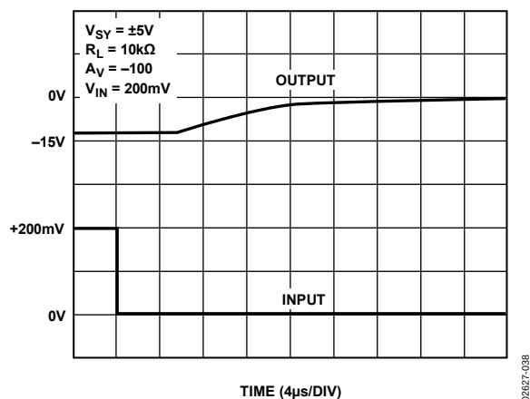
Figure 38. Positive Overtolerance Recovery
