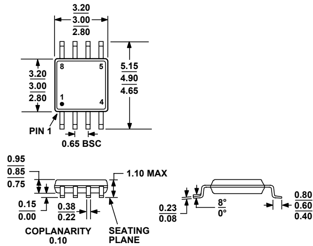
Figure 71. 8-Lead Mini Small Outline Package [MSOP] (RM-8)
