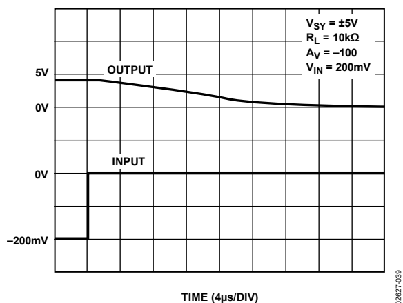
Figure 39. Negative Overtolerance Recovery
