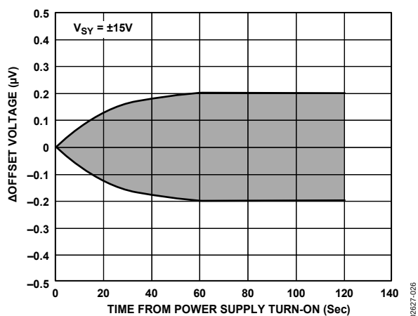
Figure 26. Warm-Up Drift
