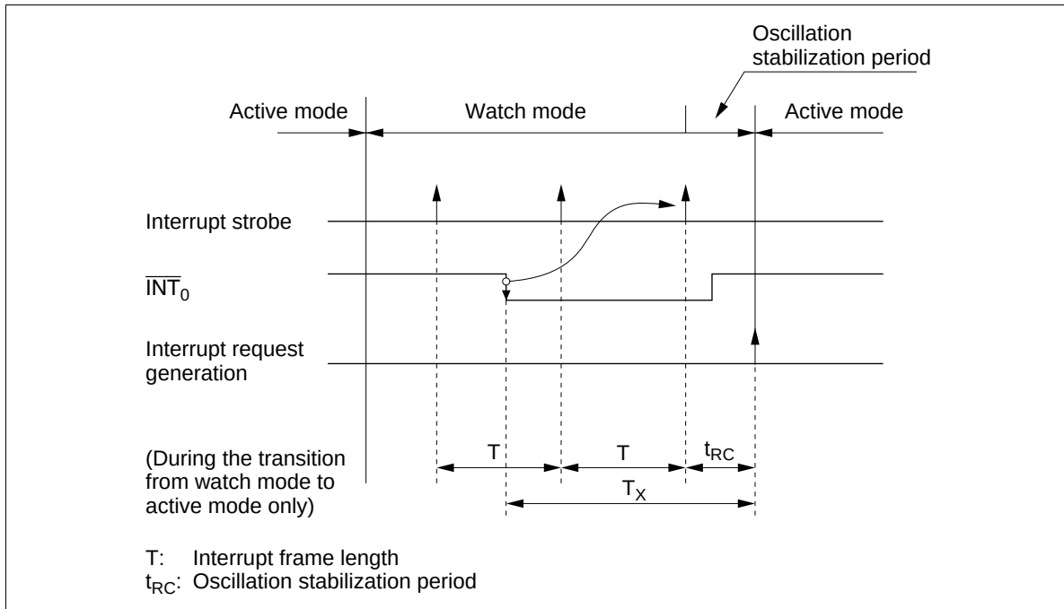
Figure 12 Interrupt Frame
