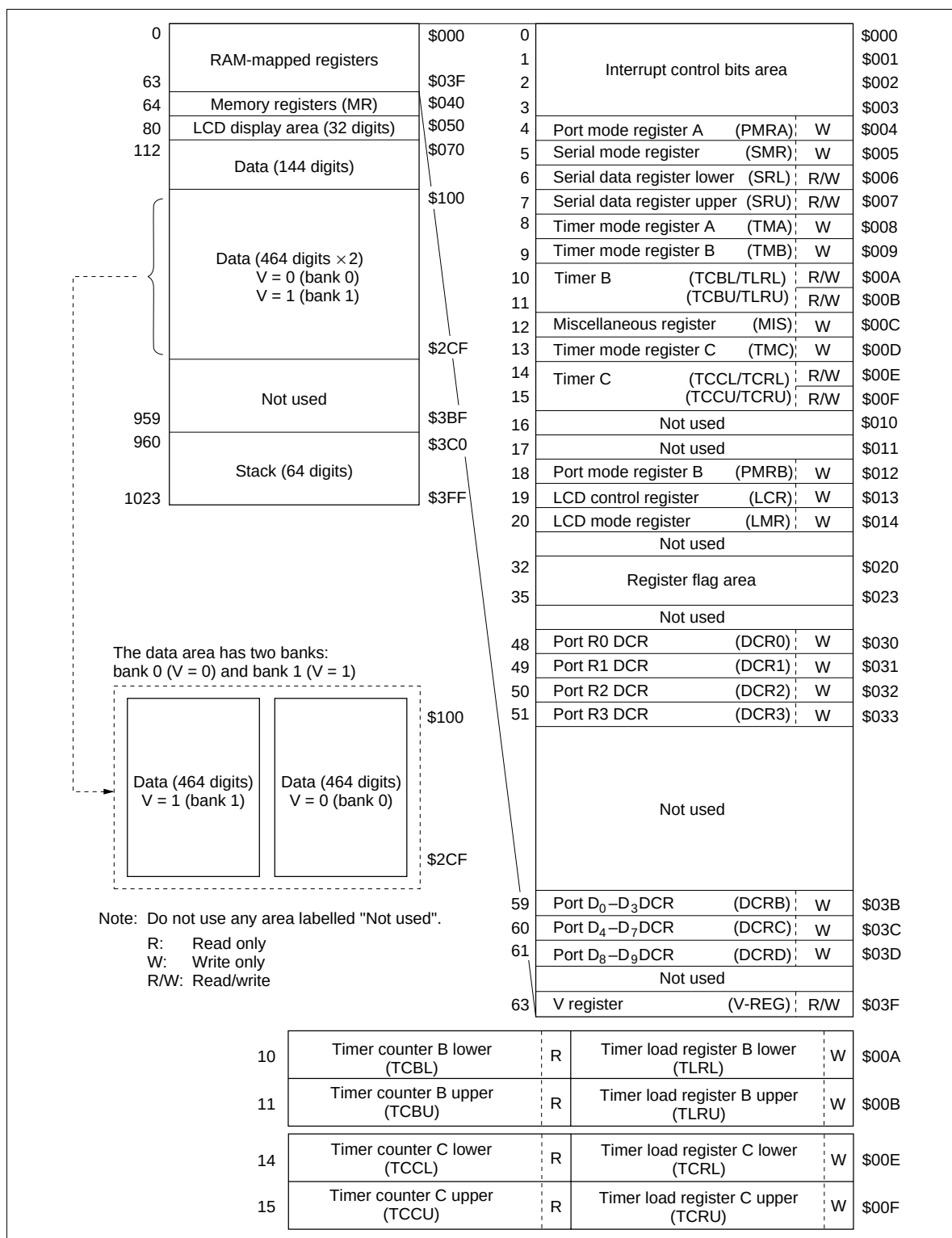
Figure 2 RAM Memory Map (1,184-digit x 4-bit)
