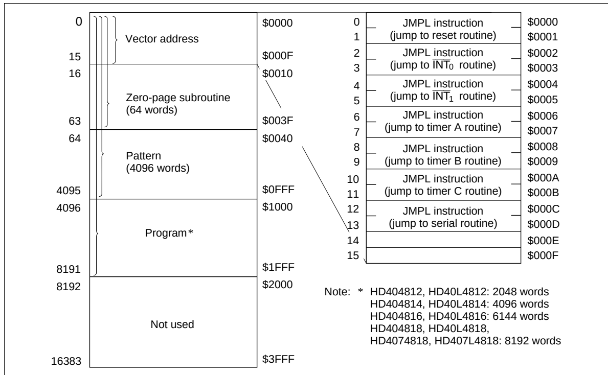
Figure 1 ROM Memory Map
